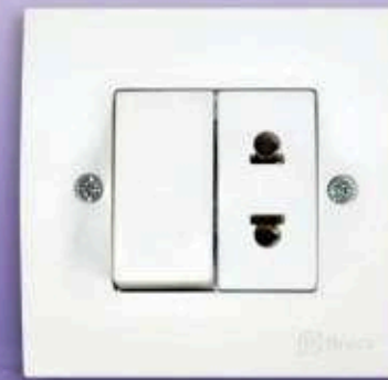
Universal Socket Outlet and Single Switch for flush mounting Art. J25361 10AX & 6A 250V~ Colors : White & Cream
