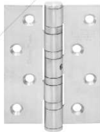
NRP ESS DL 4X3X3MM 4BB SSS Capacity (max) : 75 KG / pair Available: 4X3X4MM 4BB SSS Capacity (max) : 80 KG / pair
