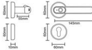
Handle Dimension
