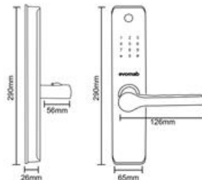
Handle Dimension
