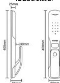
Handle Dimension
