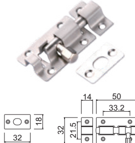
Barrel Bolt B 0901 - 2"
