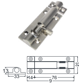
Barrel Bolt B 06
