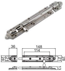
Classic Latch B 08 - 6"
