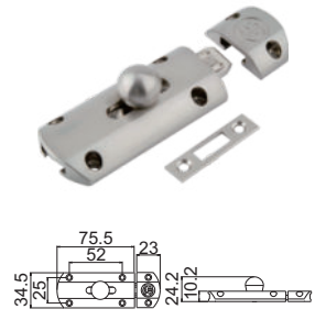
ELT Latch B 31
