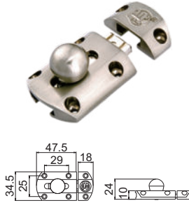
ELT Latch B 27
