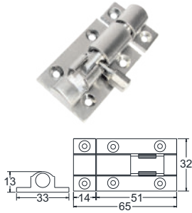
Barrel Bolt B 05
