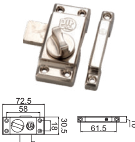
Lavatory Latch B 28
