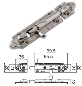
Classic Latch B 07 - 4"
