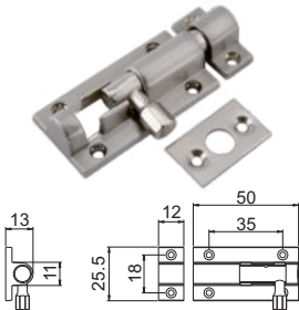
Barrel Bolt B 09 - 2"
