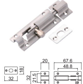
Barrel Bolt B 0902 - 3"
