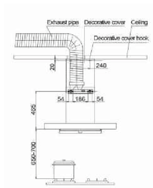
Installation Diagram
