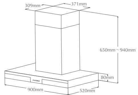
Hood EMS9020
