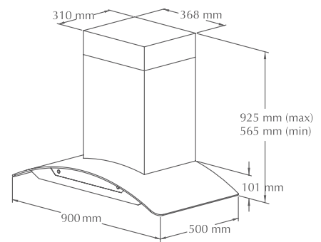
Hood EH11D
