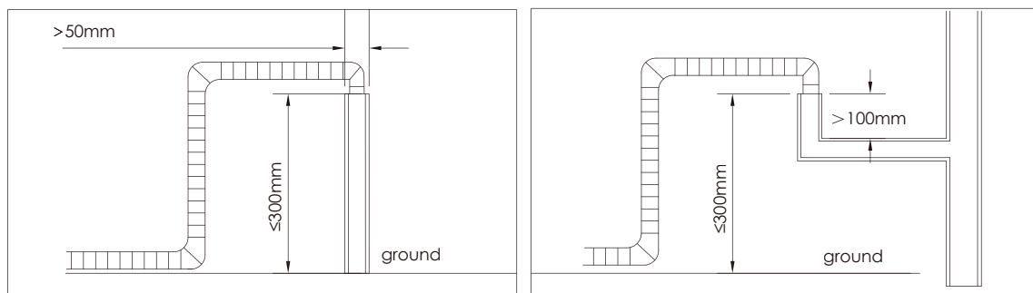
Drain-pipe installation diagram
