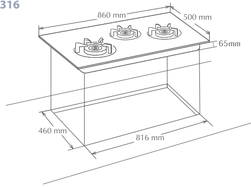
Hob GDG86316
