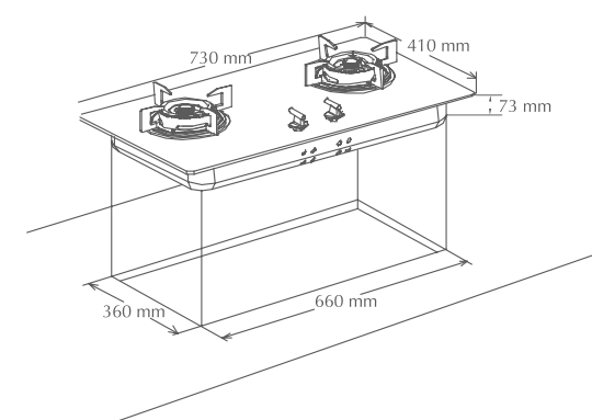
Hob FD2B
