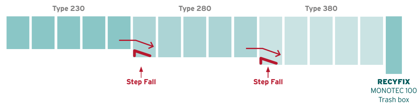
RECYFIX MONOTEC Channel 100:
