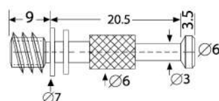
NS-10, NS-10-B Nylon Socket - M6 x 10 mm
