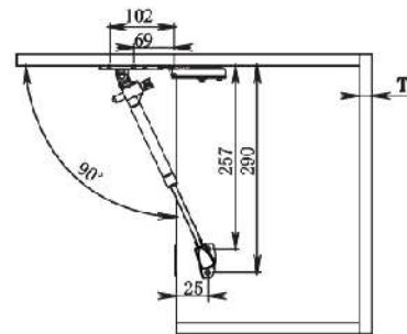
Tampak Samping
