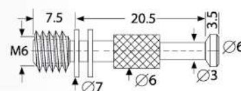
KSF-6536-11 Skrup Minifix
