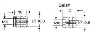
NS-10, NS-10-B Nylon Socket - M6 x 10 mm
