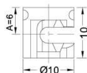
MF-15-G Casing Minifix
