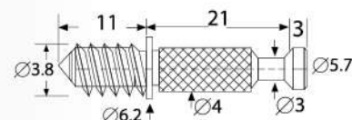
DU-62411 Skrup Minifix
