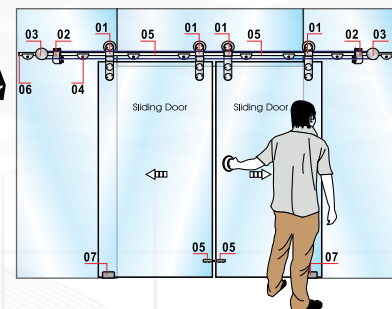
03. Synchronize Device Qty Package : 2 pcs
