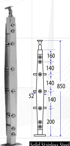
Type : RT 0104 Material : Stainless Steel Sus 304 Description : Hand-Rail for Pipe
