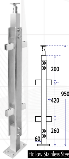
Type : RT 0115 Material : Stainless Steel Sus 304 Description : Hand-Rail for Glass
