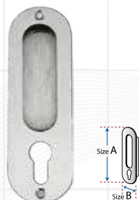
Material : Stainless Steel Type : HT 2001 Size A : 160mm, Size B : 50mm
