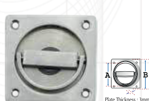
Type : HT 2117 Size : A.54mm, B.71mm Material : Stainless Steel Sus 304
