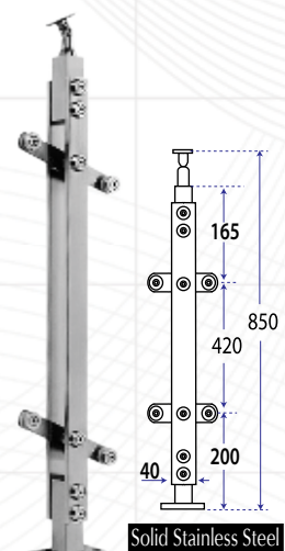
Type : RT 0103 Material : Stainless Steel Sus 304 Description : Hand-Rail for Glass
