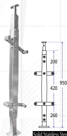
Type : RT 0114 Material : Stainless Steel Sus 304 Description : Hand-Rail for Glass
