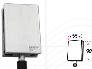
Bottom Guide RDG TH 5700~sn Type : APL 0000 Material : Stainless Steel Sus 304 Max Weight : 80 kg/door leaf
