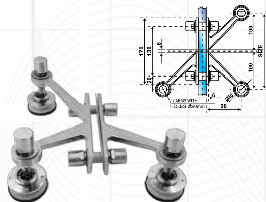
Type : BX 8317 Side : L (Left) 45° Material : Stainless Steel Sus 304
