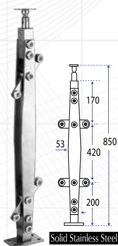
Type : RT 0106 Material : Stainless Steel Sus 304 Description : Hand-Rail for Glass
