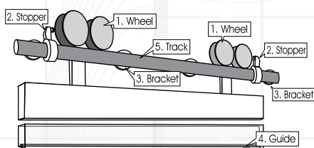
4. Guide - 1 pcs-/1set
