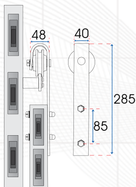
Roller Hanger Qty Package : 2 set
