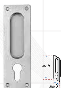
Material : Stainless Steel Type : HT 2000 Size A : 160mm, Size B : 50mm
