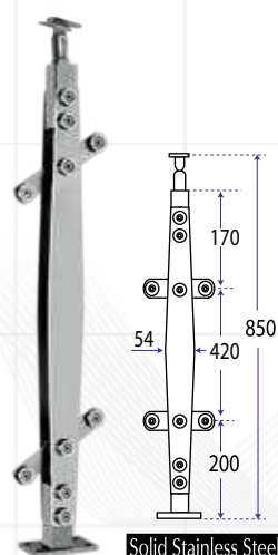
Type : RT 0111 Material : Stainless Steel Sus 304 Description : Hand-Rail for Glass
