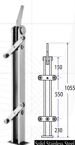
Type : RT 0118 Material : Stainless Steel Sus 304 Description : Hand-Rail for Glass
