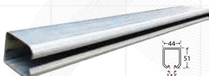
Track RAFES - S.250 kg
