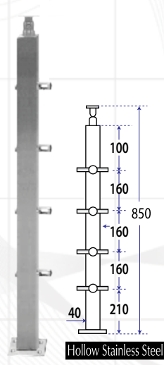
Type : RT 0117 Material : Stainless Steel Sus 304 Description : Hand-Rail for pipe
