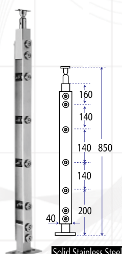
Type : RT 0102 Material : Stainless Steel Sus 304 Description : Hand-Rail for Pipe
