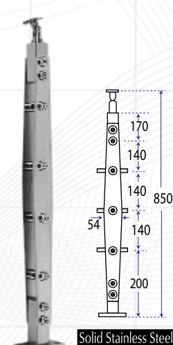
Type : RT 0110 Material : Stainless Steel Sus 304 Description : Hand-Rail for Pipe
