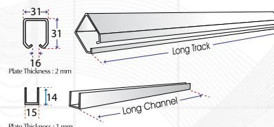
Casano - 70 kg/Set (Iron Track)
