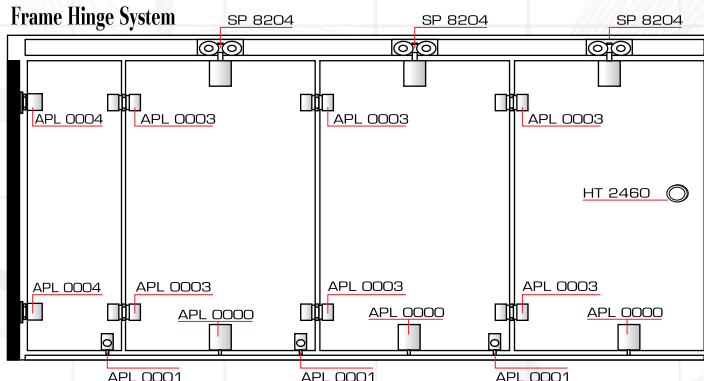
Frame Hinge System
