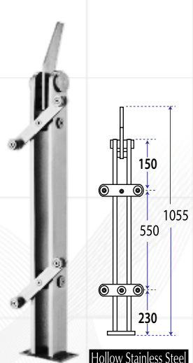
Type : RT 0105 Material : Stainless Steel Sus 304 Description : Hand-Rail for Glass
