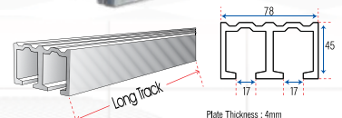
Compatible Track Double RAFES R250 kg
