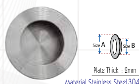
Material Stainless Steel 304 Type : HT 1974 Size A : 35mm, Size B : 19mm
