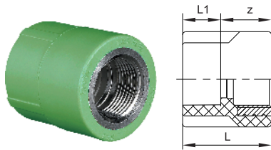
Female Thread Adapter I (Soc×Fipt with Metal Insert)
