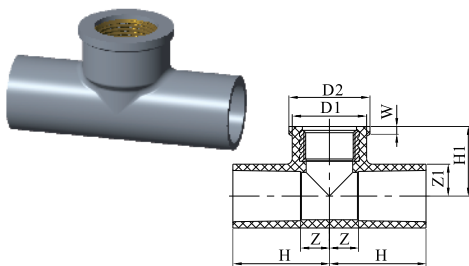
Faucet Tee With Metal Insert (AW)
