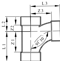
Large Radius Tee (D-LT)
