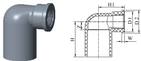
Faucet Elbow (AW)
