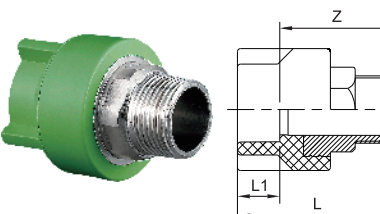
Male Thread Adapter II (Soc×Mipt with Metal Insert)
