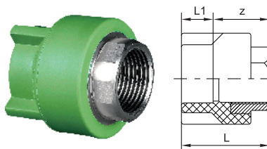
Female Thread Adapter II (Soc×Fipt with Metal Insert)
