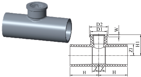
Faucet Tee (AW)
