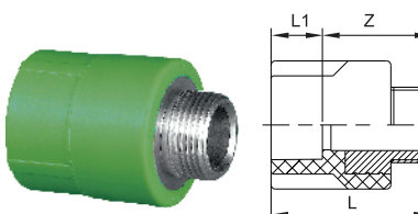
Male Thread Adapter I (Soc×Mipt with Metal Insert)
