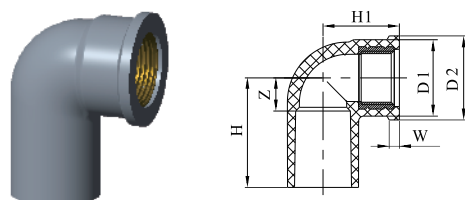
Faucet Elbow With Metal Insert (AW)
