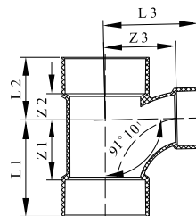
Large Radius Tee (D-LT)
