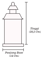
Original Lampu Taman SO-JM05 BK E27 X 1 Aluminium & Kaca
