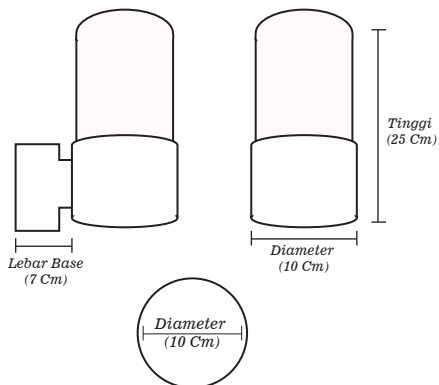
Original Lampu Dinding 1702-108 BH E27 X 1 Almunium & Kaca
