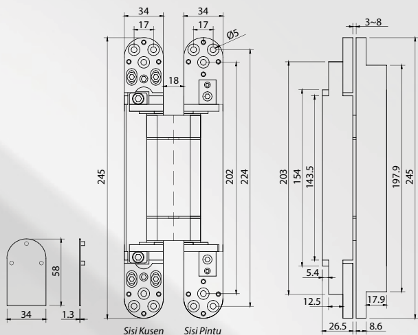
IHP 803 Natural Anodized
