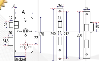
Mortice Lock Latch Series
