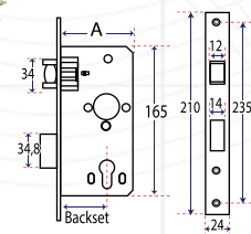
Mortice Lock Roller Series
