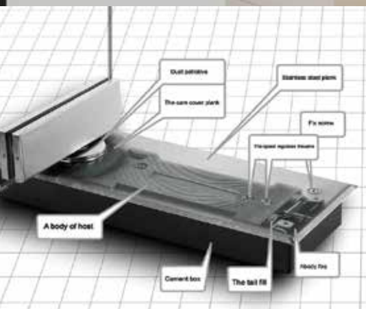
RAFES FLOOR HINGE
