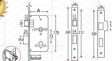
Mortice Lock Latch Series
