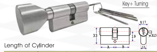
Key + Turning
