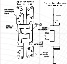
Invisible Hinge Heavy Aluminium Alloy
