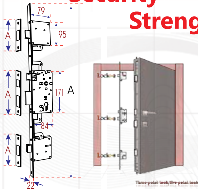
Three Point Lock Latch Series
