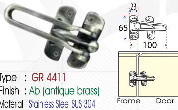
Door Guard
