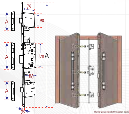
Three Point Lock Roller Series
