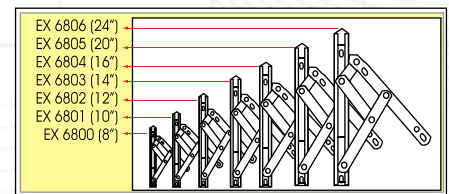
Top Hung
