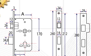
Mortice Lock Roller Series
