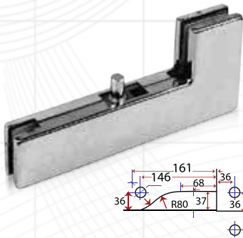
Top Patch Fitting Type : PS 3890 Material Cover : Stainless Steel Sus 304 Description : PT 40
