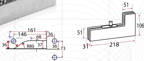
Top Patch Fitting Type : PS 3890 Material Cover : Stainless Steel Sus 304 Description : PT 40
