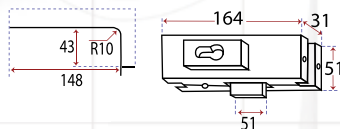
Glass Corner Lock Type : PS 3651 Material Cover : Stainless Steel Sus 304 Description : US 10
