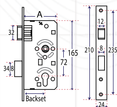
Mortice Lock Latch Series
