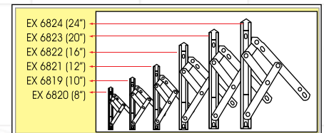
Top Hung
