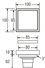
HN908 SQUARE FLOOR STRAINER
