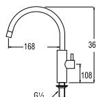
Y5475H-MDP-13 PILLAR TAP
