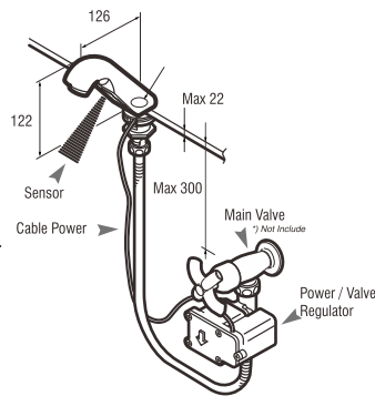
EY500 SENSOR BASIN TAP
