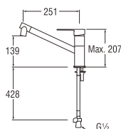
K875JDVZ-1-13 SINGLE LEVER SINK MIXER
