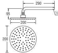
PS14-L RELAXATION WALL SHOWER
