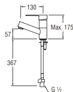
Y5475H-13 PILLAR TAP
