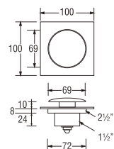
HN905 POP-UP FLOOR STRAINER
