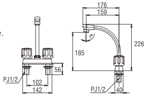
K71D-W DECK TYPE SINK MIXER
