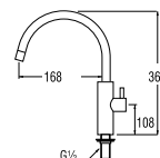
Y5475H-SJP-13 PILLAR TAP
