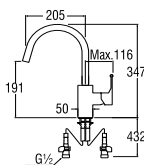
K8751JV-13 SINGLE LEVER SINK MIXER
