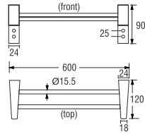
PWN531 TOWEL HOLDER
