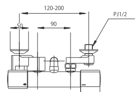
SK18C-S9 THERMOSTATIC BATH MIXER with HAND SHOWER
