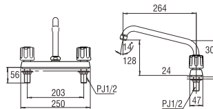
K611-W DECK TYPE SINK MIXER
