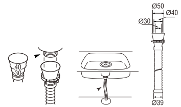
PH62-861 DRAIN HOSE 1.0, 1.5m
