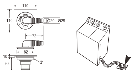
HN906 FLOOR STRAINER for WASHING MACHINE
