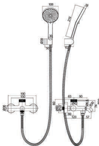
V-VT5468 GY Exposed Bath Shower Faucet with Spout and Handshower
