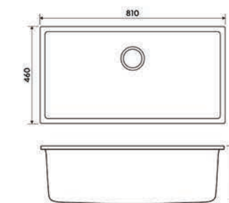
V-GE 8146M BK Undermount Granite Sink
