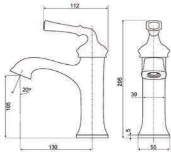
V-BT 6112 BZ Countertop Basin Faucet with Flexible Hose
