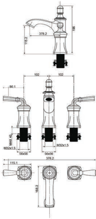
V-BT 6212 BZ 3 Hole Installation Countertop Basin Faucet with Flexible Hose
