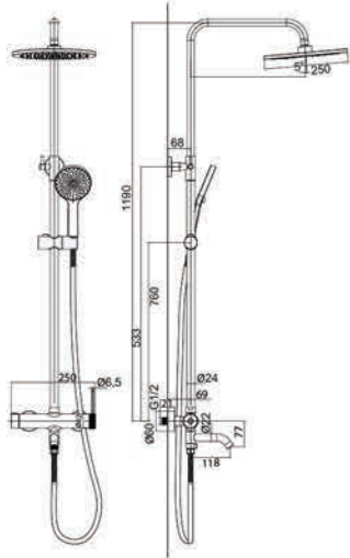
V-VT5480 GY 3 Water Output Diverter Shower Column with Overhead Shower, Handshower and Adjustable Bracket
