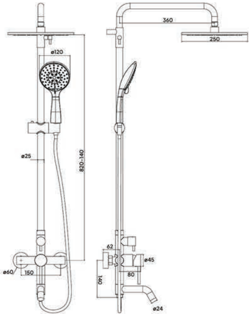
V-AE7480 BK 3 Water Output Diverter Shower Column with Overhead Shower, Handshower and Adjustable Bracket
