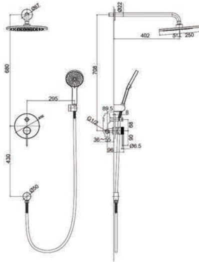
V-VT5423 GY 2 Water Output Diverter Concealed Shower Faucet with Plate, Overhead Shower with Shower Arm and Handshower with Water Outlet
